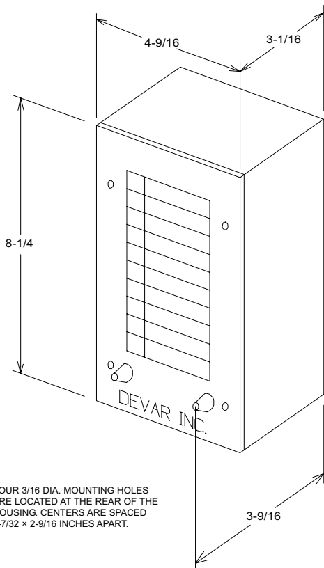
SURFACE BOX DIMENSIONS
