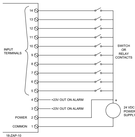
FIELD WIRING 24VDC OPERATIONAL POWER
