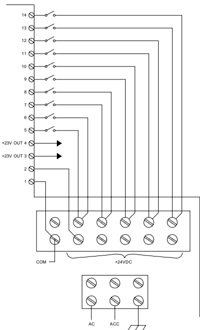
FIELD WIRING 120VAC OPERATIONAL POWER
