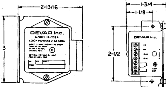
FIG. 3 GENERAL DIMENSIONS
